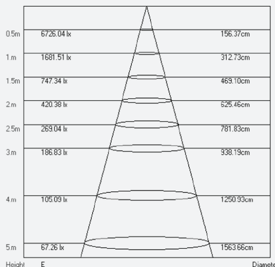
Lux-Distance Curve
